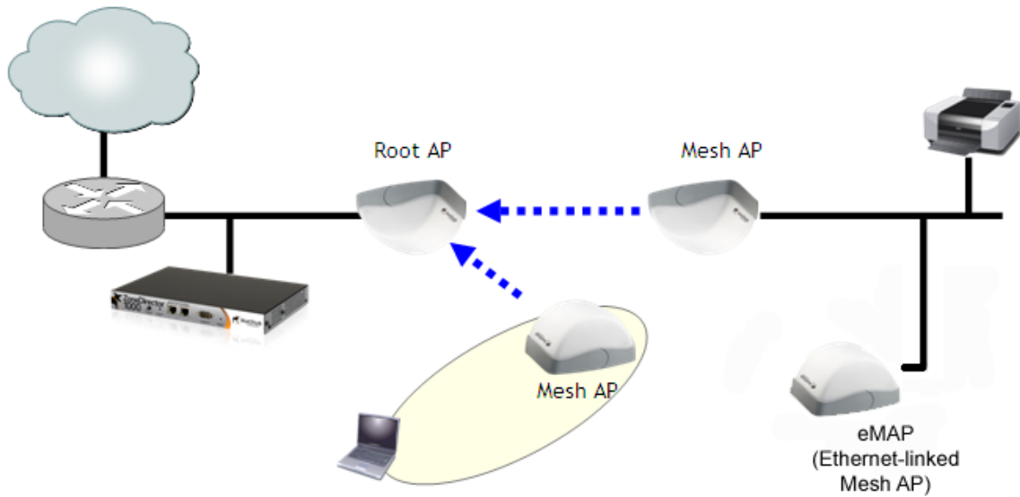
FIGURE 296 eMAP - Hybrid Mesh topology
